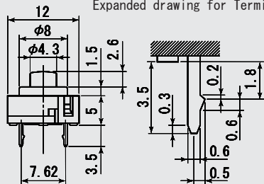
端子形状拡大詳細図 Expanded drawing for Terminal
